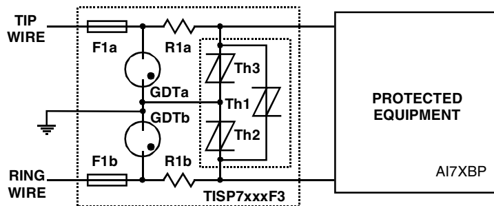
Figure 36. PROTECTION MODULE
