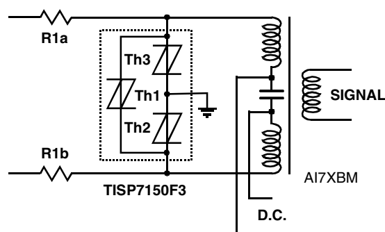
Figure 37. ISDN PROTECTION
