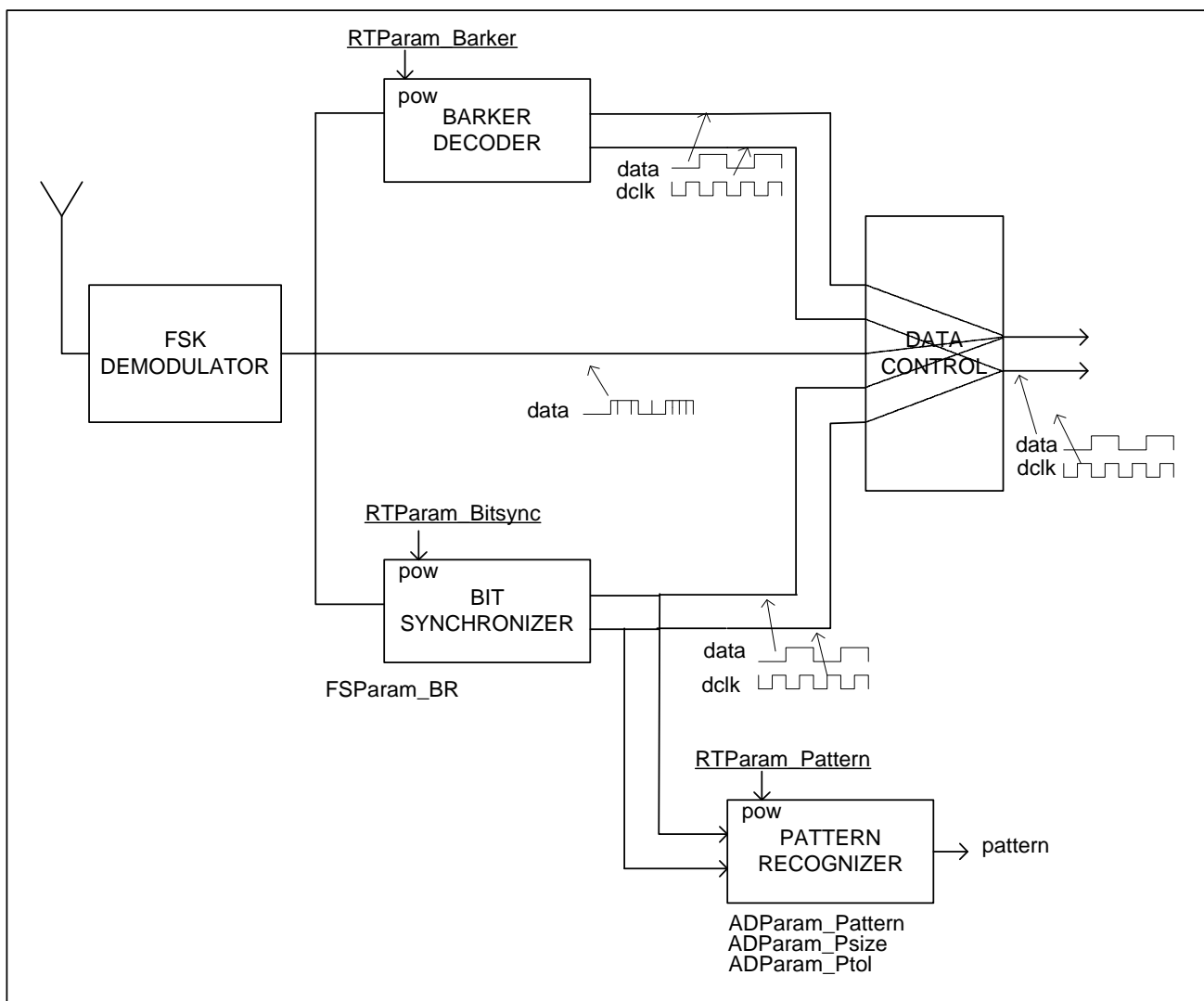
Figure 2: Demodulation architecture
