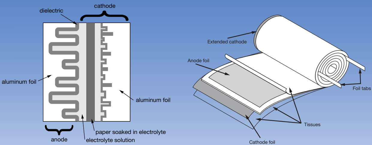
Aluminum electrolytic capacitor typical construction
