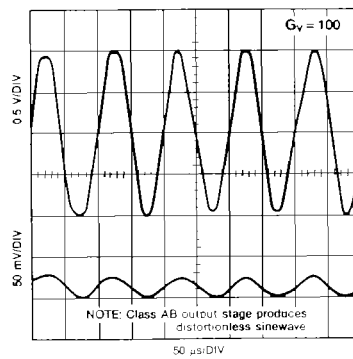
Fig. 2. Wave Response
