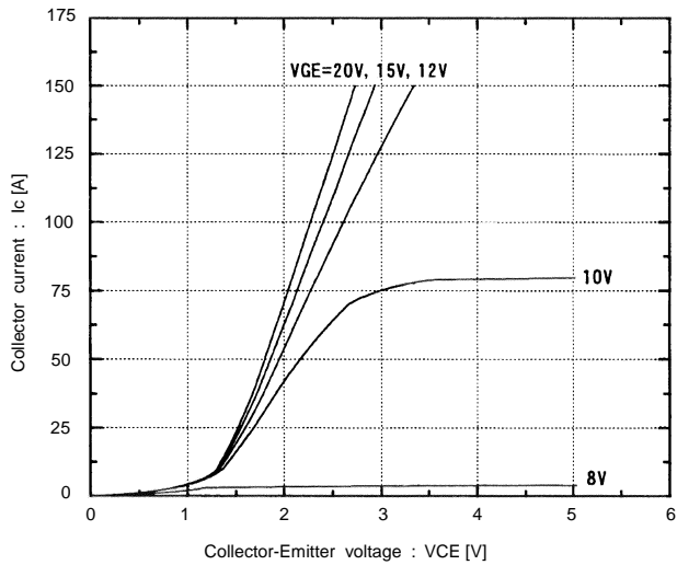
Collector current vs. Collector-Emittter voltage T J =25°C
