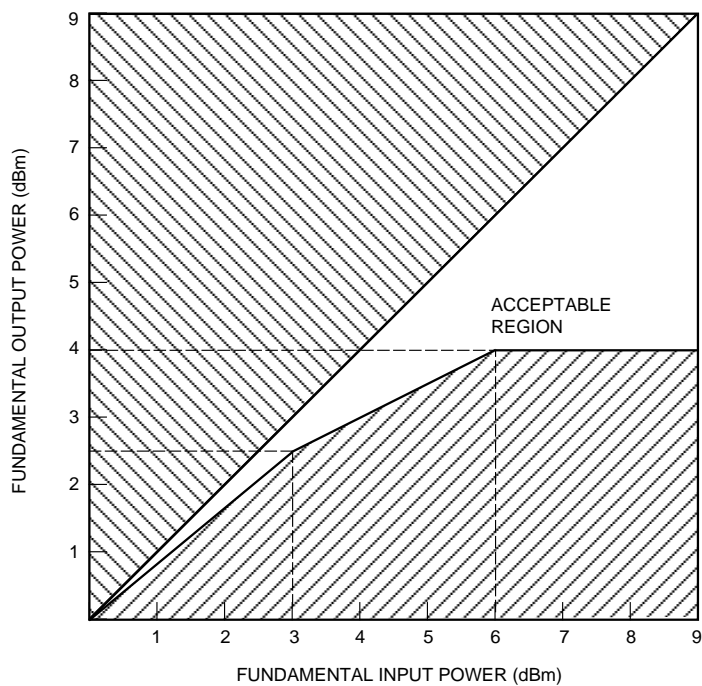
Figure 4. Overload Compression
