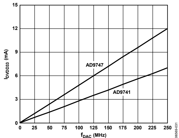
Figure 40. DVDD33 Current vs. f_{DAC}
